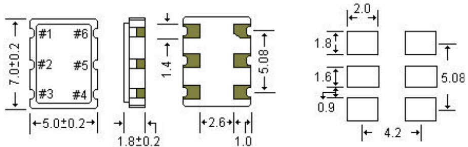
Recommended Pad Layout
